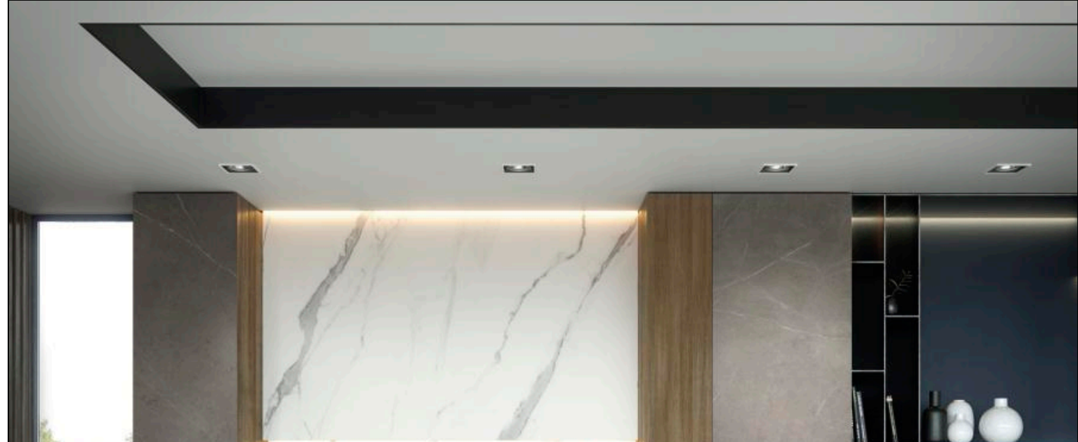
Aria (Xlight)
