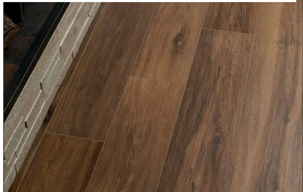
Root (Caesar)
