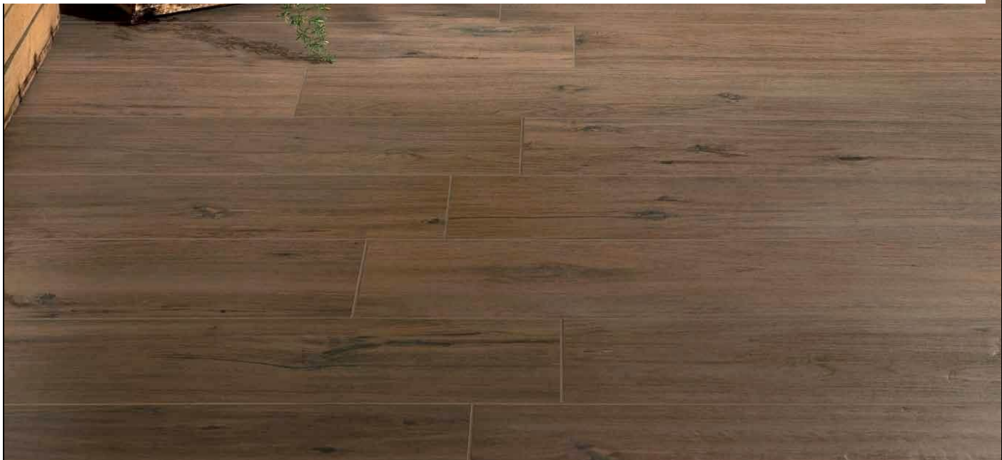
Root (Caesar)
