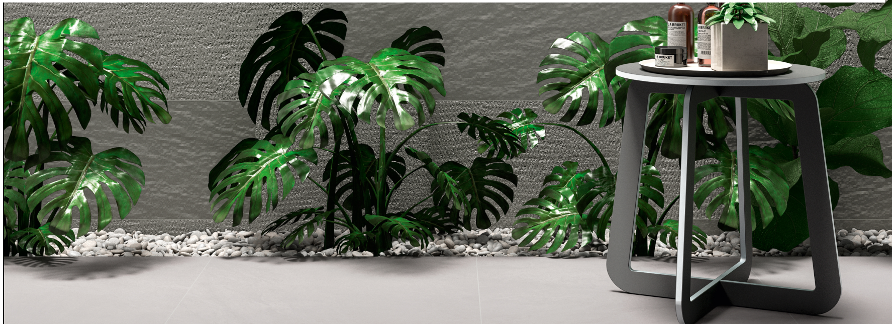
Norgestone (Novabell)
