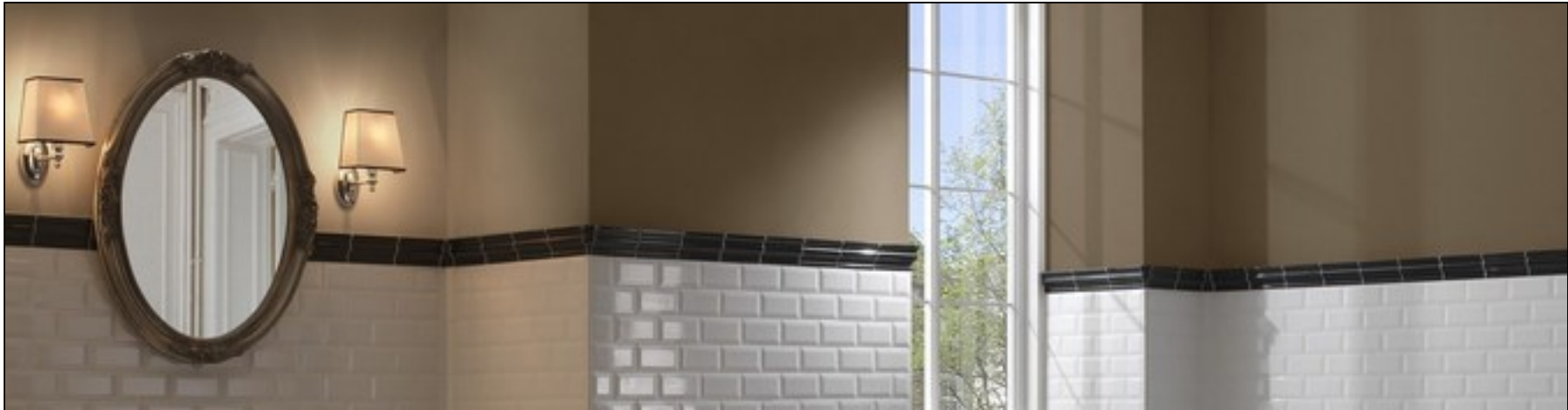
Diamante (Tonalite)
